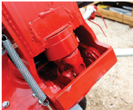
Universal connection for folding tedder arms for transport & working mode
