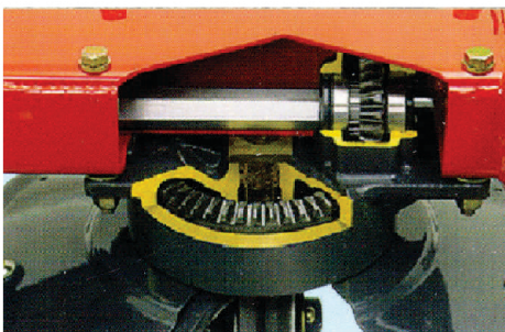
The transmission is made by exagonal shafts and sturdy pinion lubricated with grease
